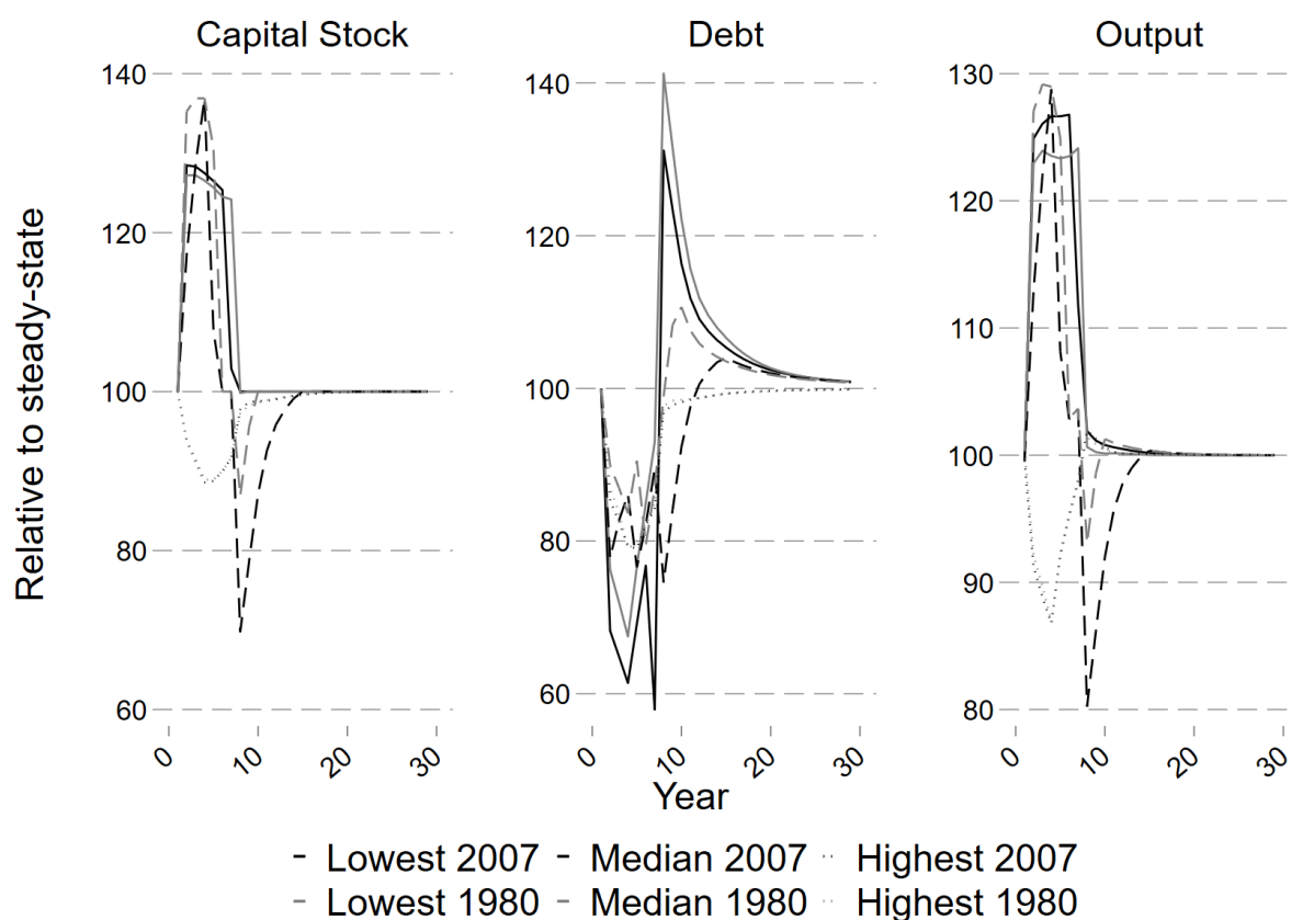
Figure 4: Recovery of aggregate variables from a financial crisis under different firm-size distributions, split by quintile of capital
