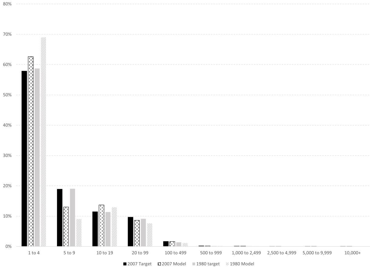
Figure 2: Comparison of firm-size distribution targets and calibrated model results
